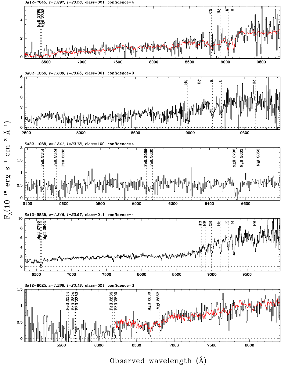
Fig. 9.— Representative GDDS spectra in the range 1.297 < z < 1.388 . In cases where it is useful for identifying the redshift, the SDSS luminous red galaxy composite is overlain on the spectrum (in red) as in Fig. 7. Masked regions in spectra are indicated using horizontal bars. See the caption of Figure 7 for details. The spectrum of SA12-7045 and SA12-8025 have been binned to a pixel size of 8 \text{ \AA} .
