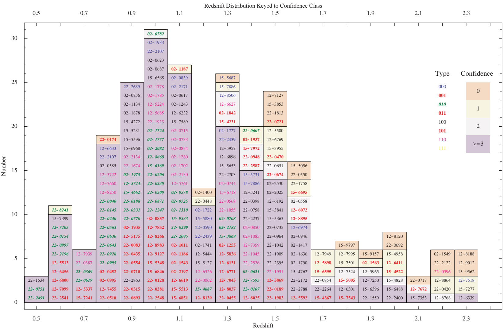
Fig. 16.— Master summary of the GDDS. This histogram illustrates the redshift distribution of our sample as a function of confidence class and spectral type. Bar colors indicate confidence in the redshifts, keyed to the system defined in Table 2. Individual objects are labeled in each histogram and sorted by spectral class. Label colors are keyed to spectral class.
