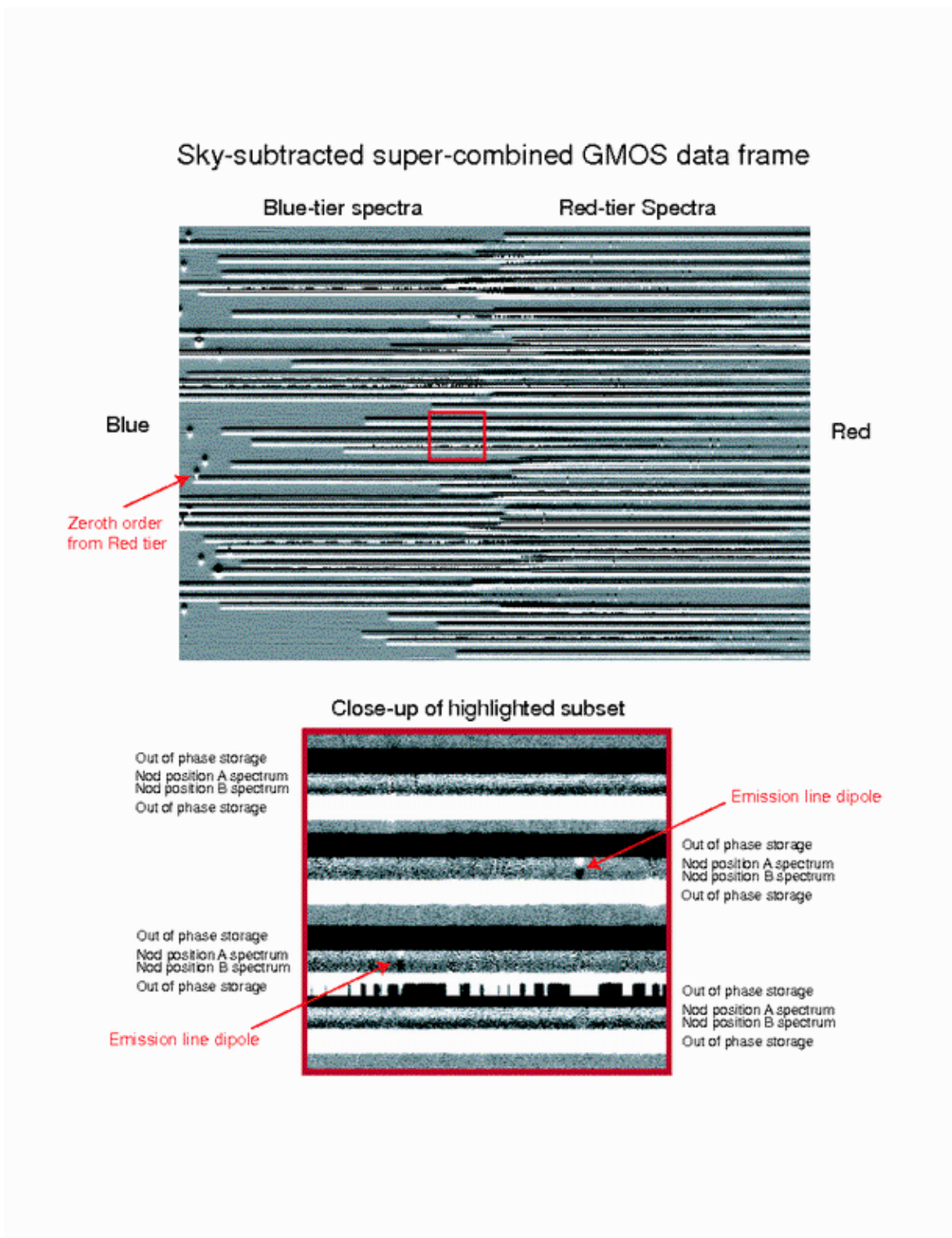
Fig. 19.— An image showing a sky-subtracted “supercombined” frame for the GDDS-SA22 field. Object spectra are sandwiched between positive and negative sky spectra on the mask. The lower half of the figure shows a magnified view of the small rectangular region near the center of the mask image. This magnified view shows subsets of four spectra with characteristic positive and negative continua and emission lines. Note that for clarity we have reversed the GMOS data format to show bluer wavelengths to the left.
