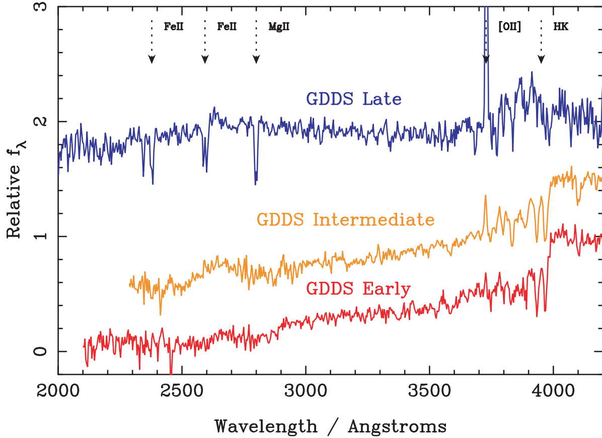
Fig. 17.— The three GDSS template composite spectra used for redshift comparison. These were constructed internally from our sample from galaxies covering a range 0.6 < z < 2 with high confidence redshifts. The templates are plotted at 3.5\text{\AA} per pixel resolution and are normalized to unity at 4200\text{\AA} , they are offset vertically in the plot for clarity. Some of the more common features are marked. Only the UV portion of the templates is shown.
