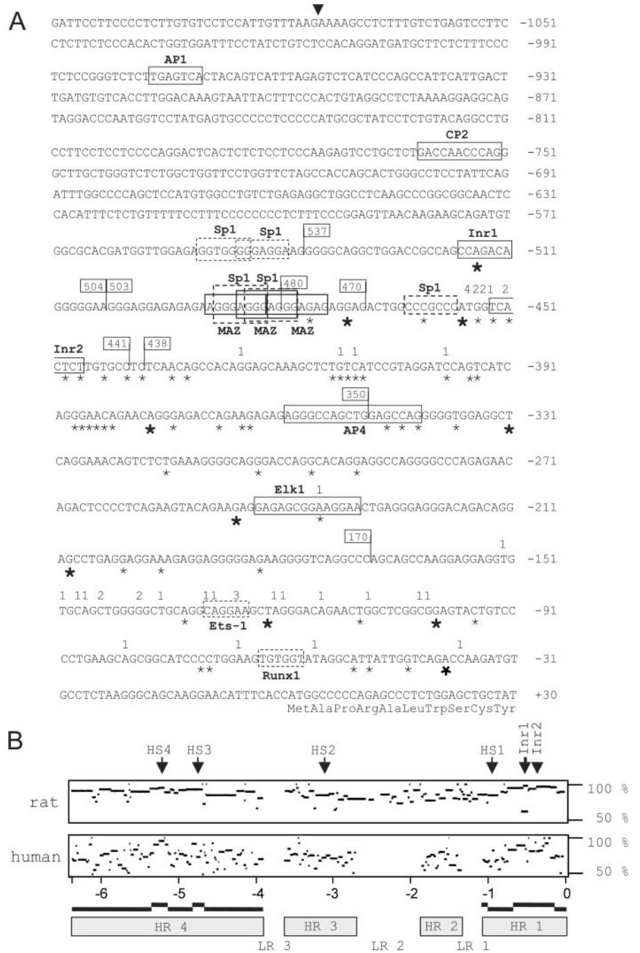
FIG. 1. Analysis of the 5'-flanking region. A , determination of transcription initiation sites of Emilin1 . The figure shows the proximal 1110 nucleotides. Numbers above the sequence mark the 5'-end of RACE clones and indicate the number of clones with the same end. Asterisks below the sequence denote the position of the 5'-end of bands produced by RNase protection; small and large asterisks denote faint and strong bands, respectively. The sequences of putative transcription factor binding sites are boxed: boxes with continuous lines refer to binding sites conserved in the three species examined (mouse, rat, and human); boxes with dashed line delimit binding elements detected only in the mouse sequence. Numbered flags define the position of the 5'-end ( right flag ) or 3'-end ( left flag ) of deletion constructs defined in Fig. 2. Arrowhead marks the 5'-end of the exonuclease deletion identified in this paper as the 1.1-kb fragment. B , percent identity plot of the 5'-flanking region of murine Emilin1 gene with the corresponding rat and human Emilin1 genomic sequences, generated by pairwise alignment with the MultiPipMaker program. The percentage sequence identities (50–100%) are shown on the y axis. The scale (in kb) on the x axis refers to the position in the murine sequence. Stretches of sequence identity are indicated by horizontal lines, corresponding to length and percentage of nucleotide sequence identity. Position of the Initiator sequences ( Inr1 and Inr2 ) and of the DNase I-hypersensitive sites ( HS1 to HS4 ) is indicated by vertical arrows. The existence of three regions of low sequence (<50%) similarity ( LR1 to LR3 ) defines four regions of high similarity ( HR1 to HR4 ). The presence of peaks of very high sequence similarity can further divide high similarity regions into subregions, indicated in the figure by alternating thick lines.
