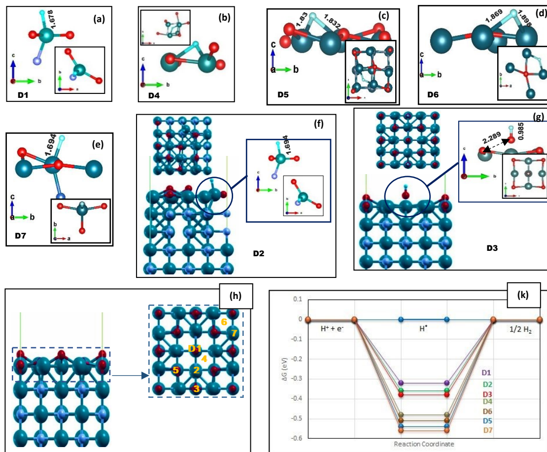
Fig. 2. The VO/VN configuration after H adsorption, where all the N atoms on the topmost layer are replaced with O atoms. (a)-(g) show the local structure of adsorbed hydrogen on top of the surface, while D1-D7 sites are marked on (h) by orange color. The top and lateral views of (a)-(e) are shown in Fig. S6. The bonding lengths are reported in Å unit. (k) shows a comparison between the corresponding H adsorption energies reported in Table 1.
