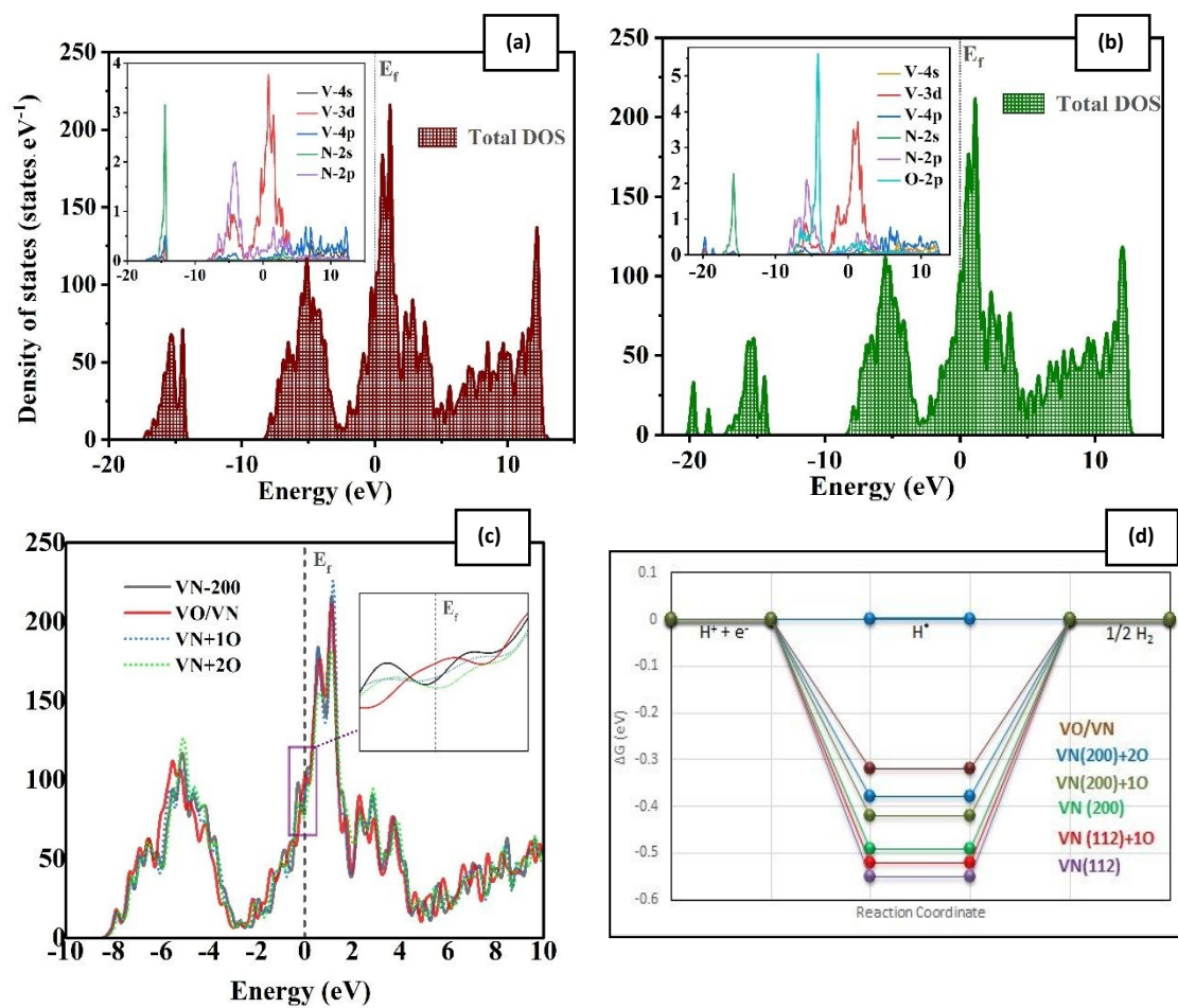
Fig. 3 Density of States plots for (a) pure VN (200), and (b) VO/VN surfaces, where the insets represent the Partial DOS plots. The Fermi level is put on zero. A comparison between the total DOSs near the fermi level is represented in (c), and (d) denotes a comparison between the Gibbs Free energies related to the best catalytic performance of surfaces.
