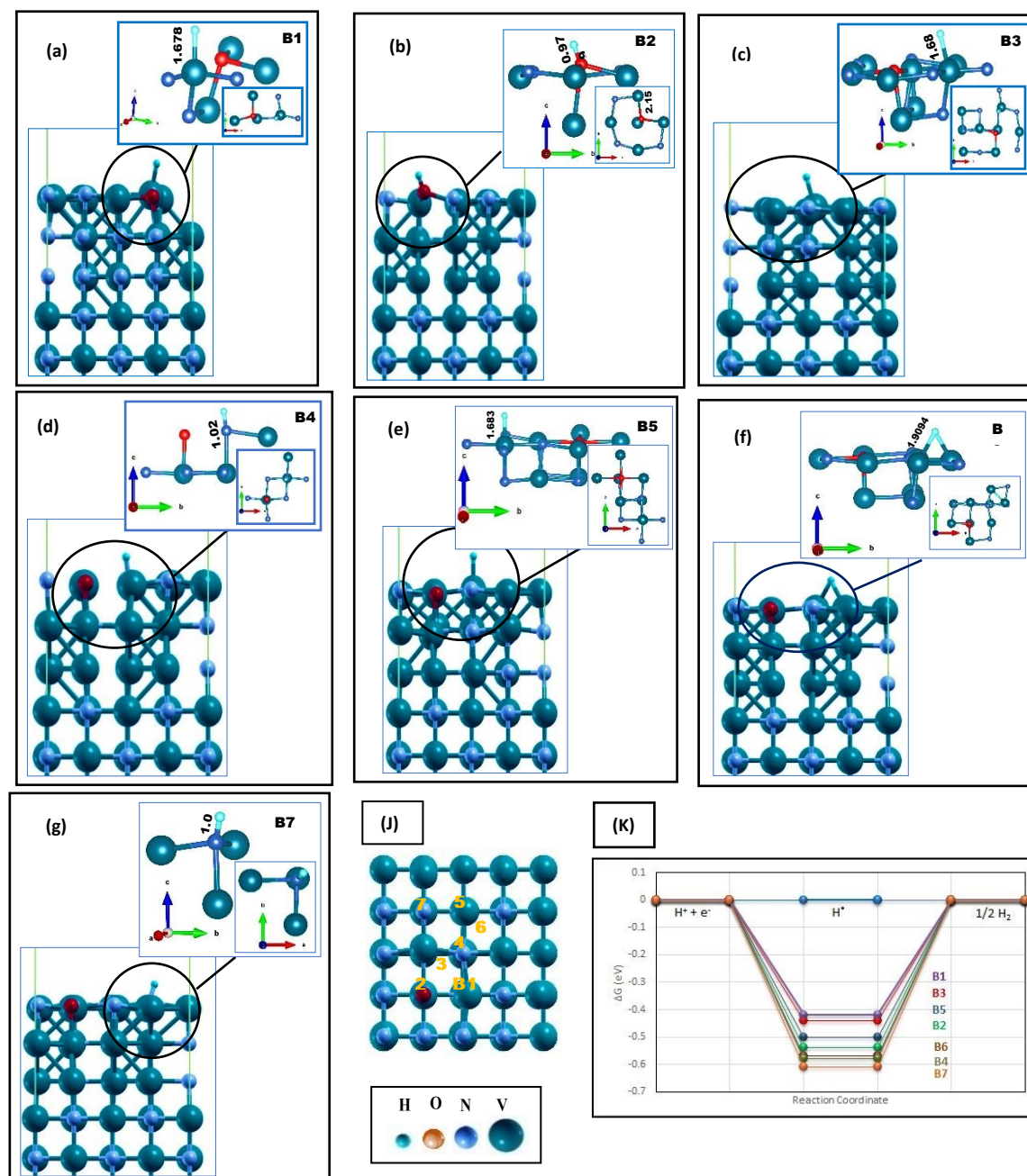
Fig. 1. Hydrogen adsorption on O-doped VN (200) in lateral and local configurations, where H^* is initially located on (a) top of V in direct vicinity of oxygen (b) top of oxygen, (c) hollow site near the oxygen, (d) top of N in direct vicinity of O, (e)-(g) top of V, N and hollow space in the indirect neighboring of O, respectively. The H bonding lengths are written in Å unit on each figure. The H^* adsorption sites are marked as B1-B7 represented in (k), and (j) denotes a schematic comparison between the free energies reported in Table 1. In all figures, the surface index is put in parallel with the c axis. V, N, O and H atoms are represented by aquamarine, grey, red and blue color balls, respectively.
