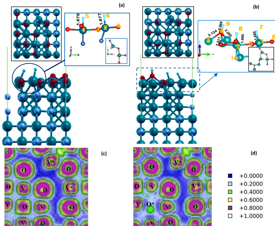
Fig. 4. Hydrogen adsorption on VO/VN surface at low H convergence. (a) and (b) represent the 1/4ML and 3/8ML hydrogen coverage of the surface, respectively. The corresponding Electron Localization Function (ELF) plots are reported in (c) and (d). An asterisk is placed on some sites to indicate that these atoms are linked to hydrogen.
