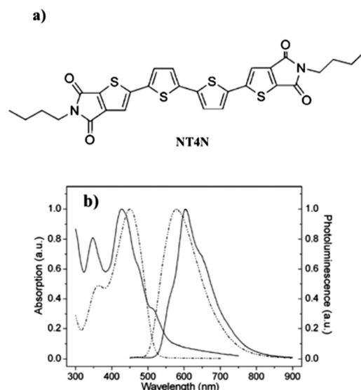
Fig. 5 (a) Molecular structure (b) normalized absorption and emission of NT4N solution (CH 2 Cl 2 , 4 × 10 -5 M, dashed line) and film (100 nm thick, solid line). Adapted from ref. 63 with permission from the Royal Society of Chemistry.
