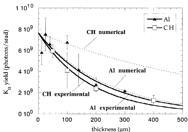
Fig. 3. Experimental and numerical results for Mo K_\alpha yield versus target thickness at I_L = 1-2 \times 10^{19} \text{W}/\text{cm}^2 . The lines are exponential interpolations of data. Error bars on experimental points are given by the standard deviation of results. Where there are no error bars, a single experimental point has been obtained at the corresponding thickness.
