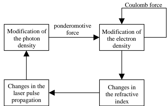
Figure 8: Schematic of laser-plasma interactions.
