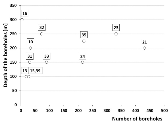
Fig. 5. Features of the BTES of the surveyed 5GDHC networks classified via ID number.
