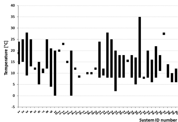
Fig. 6. Supply temperature variation of the network for the surveyed 5GDHC systems.
