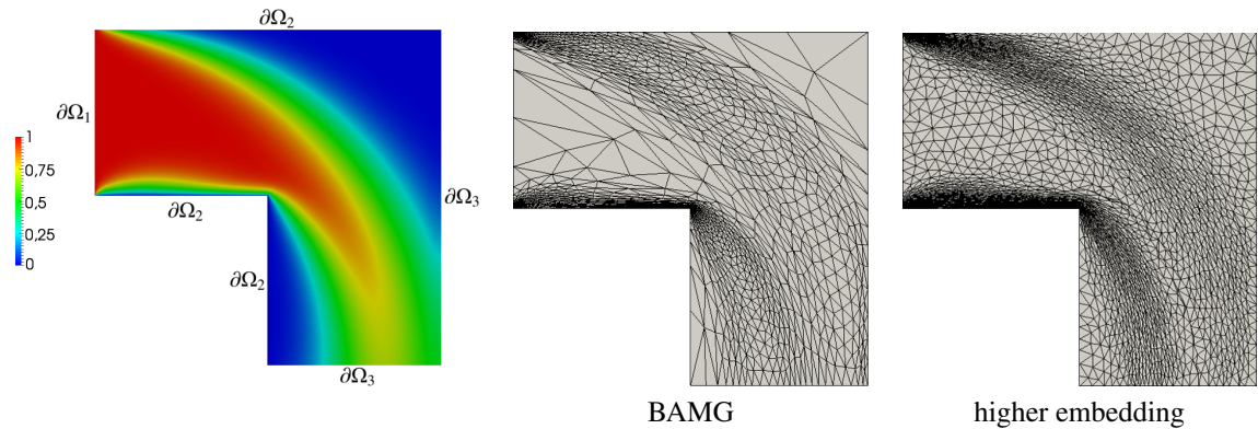
Fig. 10. The reference solution, left, the adapted mesh with BAMG, middle, the one obtained with the higher dimensional embedding, right.
