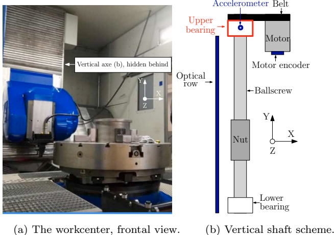
Fig. 3. Schematic of the workcenter with upper bearing highlighted.
