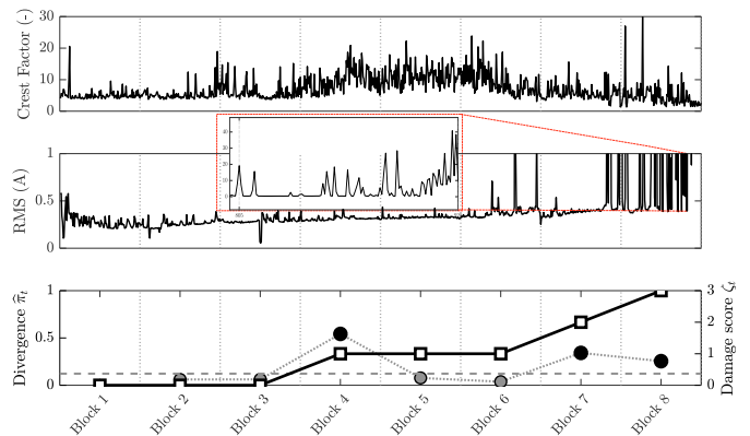
Fig. 10. Results of the proposed monitoring scheme on the workcenter bearing vibration data.
