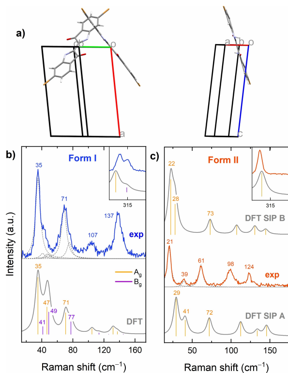
Figure 7. a) Crystal structures of Form I (left) and Form II (right) of tyrian purple; b,c) Experimental and DFT-vdW simulated Raman spectra of Form I and II in the range 10–170 \text{cm}^{-1} . Vertical bars of height proportional to the intensity of the mode identify the calculated values, with colour codes yellow and violet for modes of symmetry A_g and B_g , as indicated. Insets: experiments and calculations for a doublet at 309/315 \text{cm}^{-1} of Form I and the corresponding single band of Form II. Such a difference can be taken as diagnostic of the different number of molecules per unit cell in their structures.
