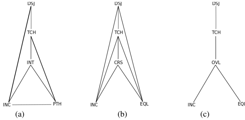
FIGURE 2. OCN graph of polygon-polyline (a), polyline-polyline (b), and polygon-polygon (c) topological relationships
