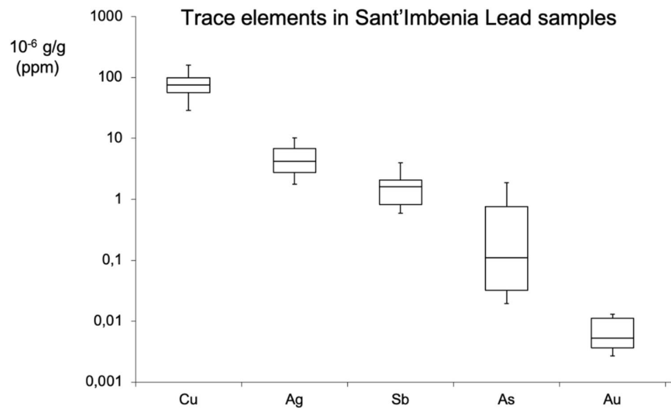
Fig. 4 Boxplot showing trace element distributions of Sant’Imbenia lead samples measured with neutron activation analysis (for detail see Romanò 2016)
