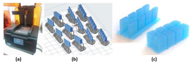
FIGURE 7. Picture of the fabrication process of UCs arrangement by means of SLA. a) Formlabs Form3 3D printer; b) Sample models pre-processing with Formlabs PreForm; c) Samples after IPA washing and UV curing.
