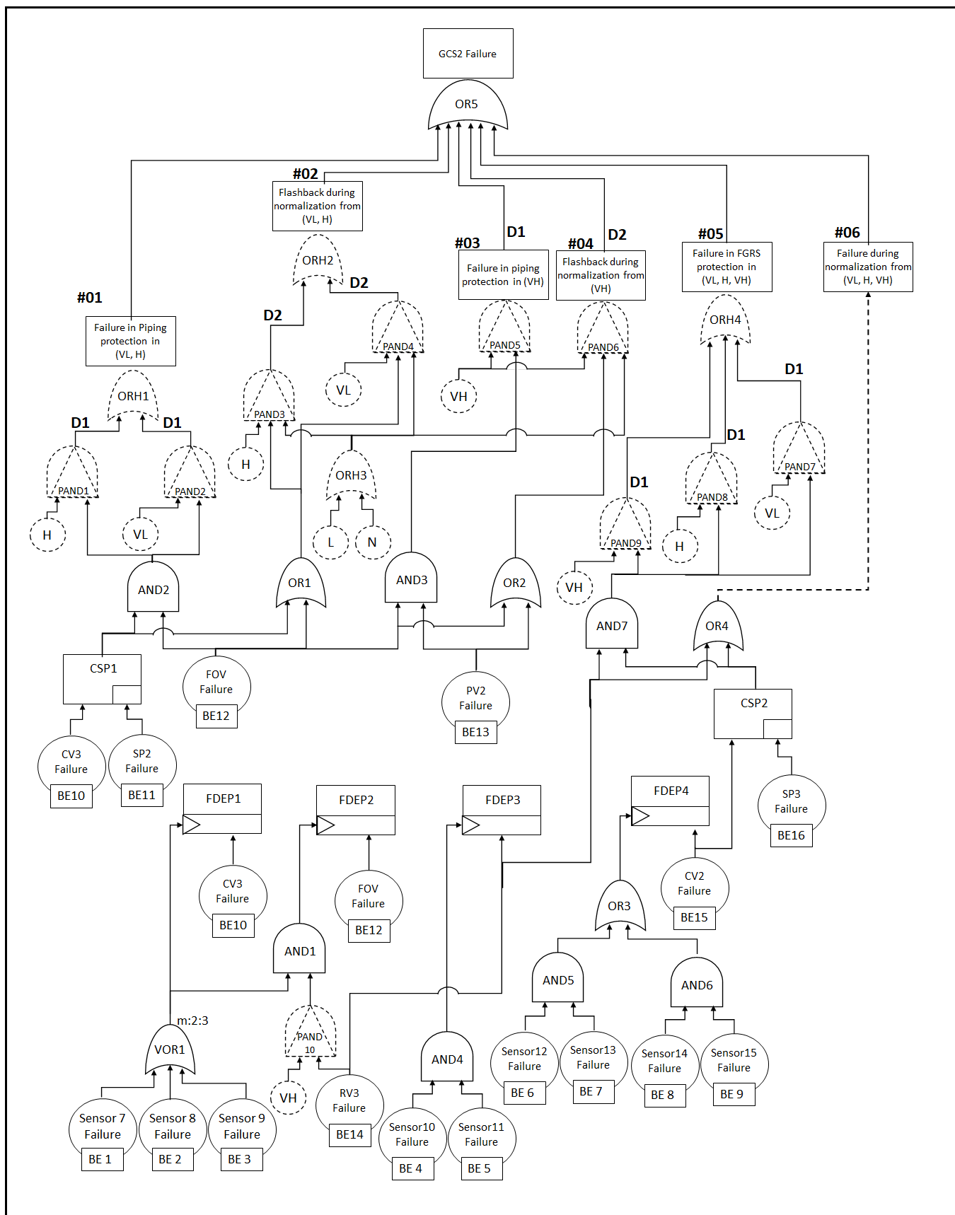
FIGURE 10 GCS2. Hybrid DFT
