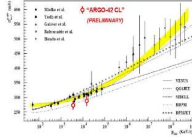
Figure 6. Inelastic cross section \sigma_{p-Air} preliminarily measured with a data sample of ARGO-42 (open circles) as compared with other measurements and theoretical estimates.
