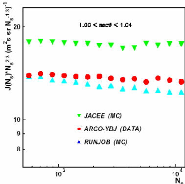
Figure 3. The ARGON- YBJ strip size spectrum as compared with the expected ones, namely with the RUNJOB and JACEE composition models (see text).
