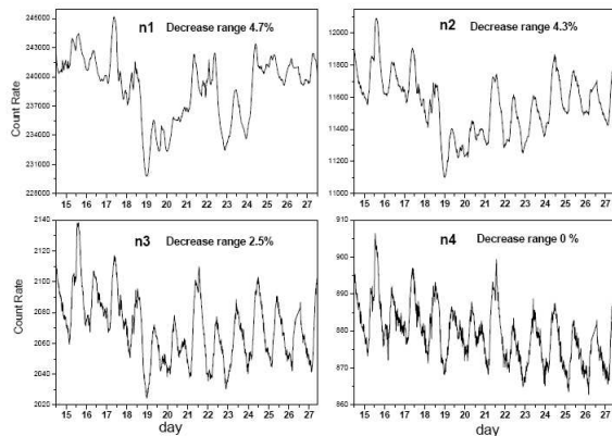
Figure 4. Counting rates summed up for 12 clusters in ARGON- YBJ from January 15th to 27th, 2005
