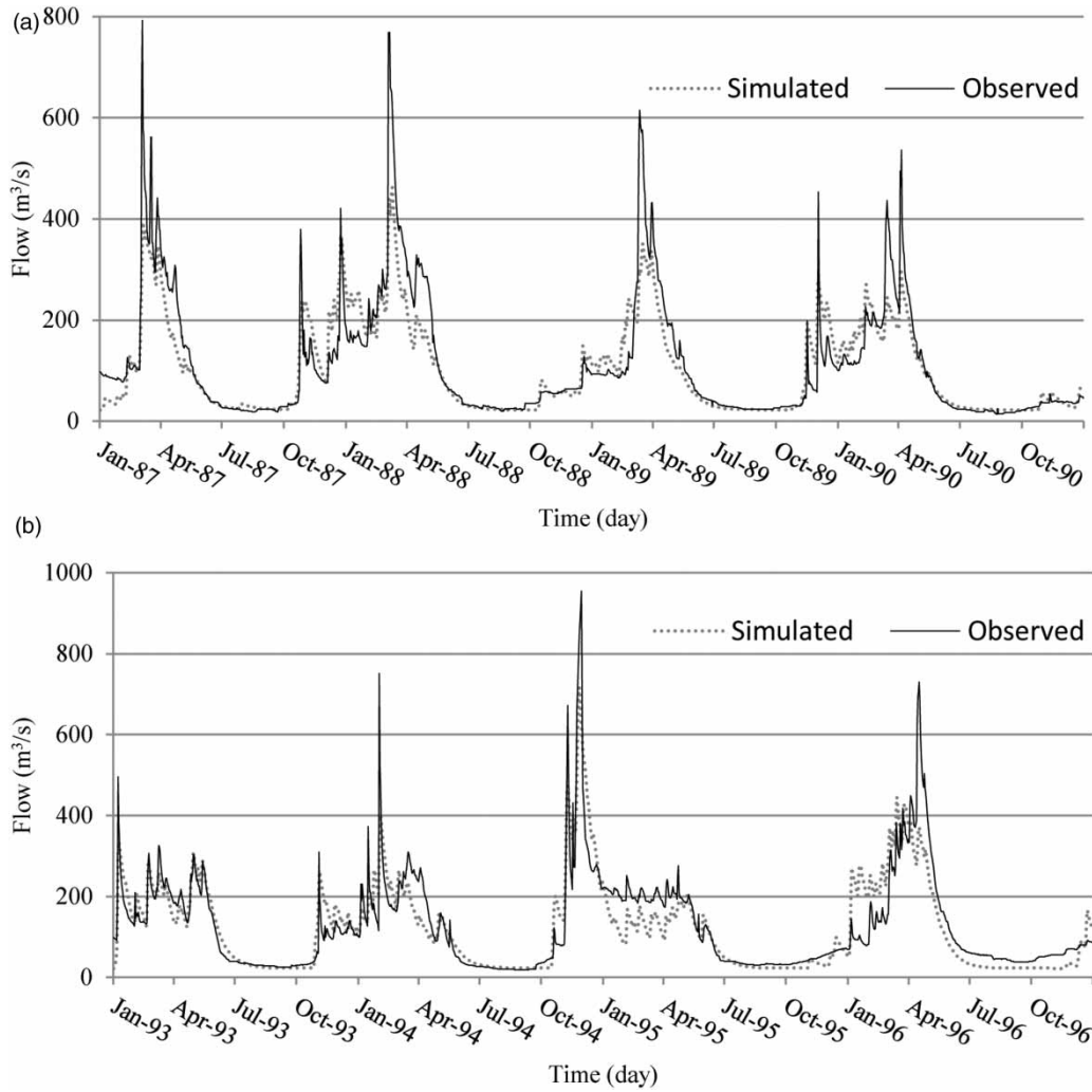
Figure 5 | Comparison of observed and simulated daily inflow to Seimareh Dam (calibration period: (a) and validation period: (b)).
