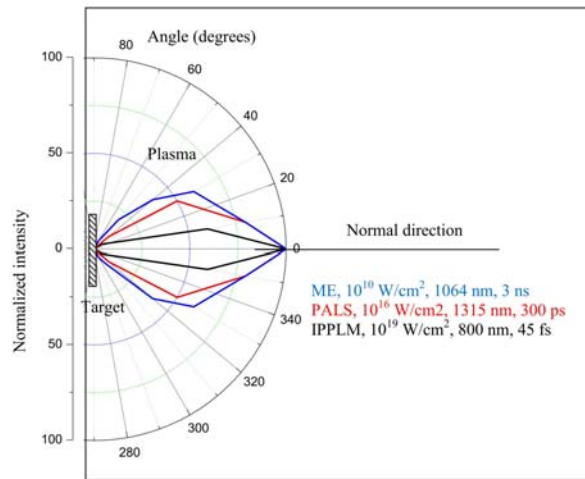
Fig. 8. Comparison of the total ion angular emission from PE for the lasers intensities at 10 10 (the widest), 10 16 and 10 19 (the narrowest) W/cm 2 laser intensity.
