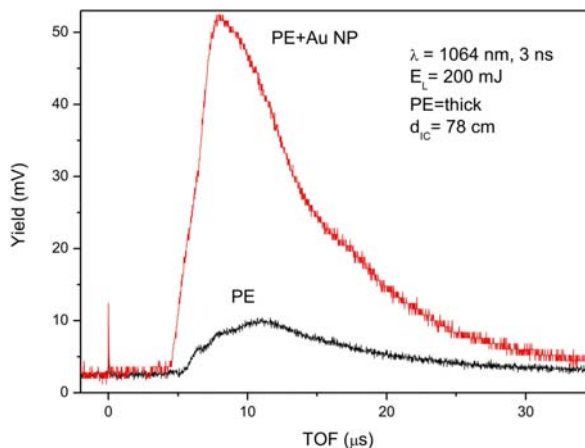
Fig. 3. TOF spectra comparison of ions accelerated at low laser intensity 10^{10} \text{W}/\text{cm}^2 , 3 ns irradiating pure PE and PE + Au NP and detecting in BPA regime.
