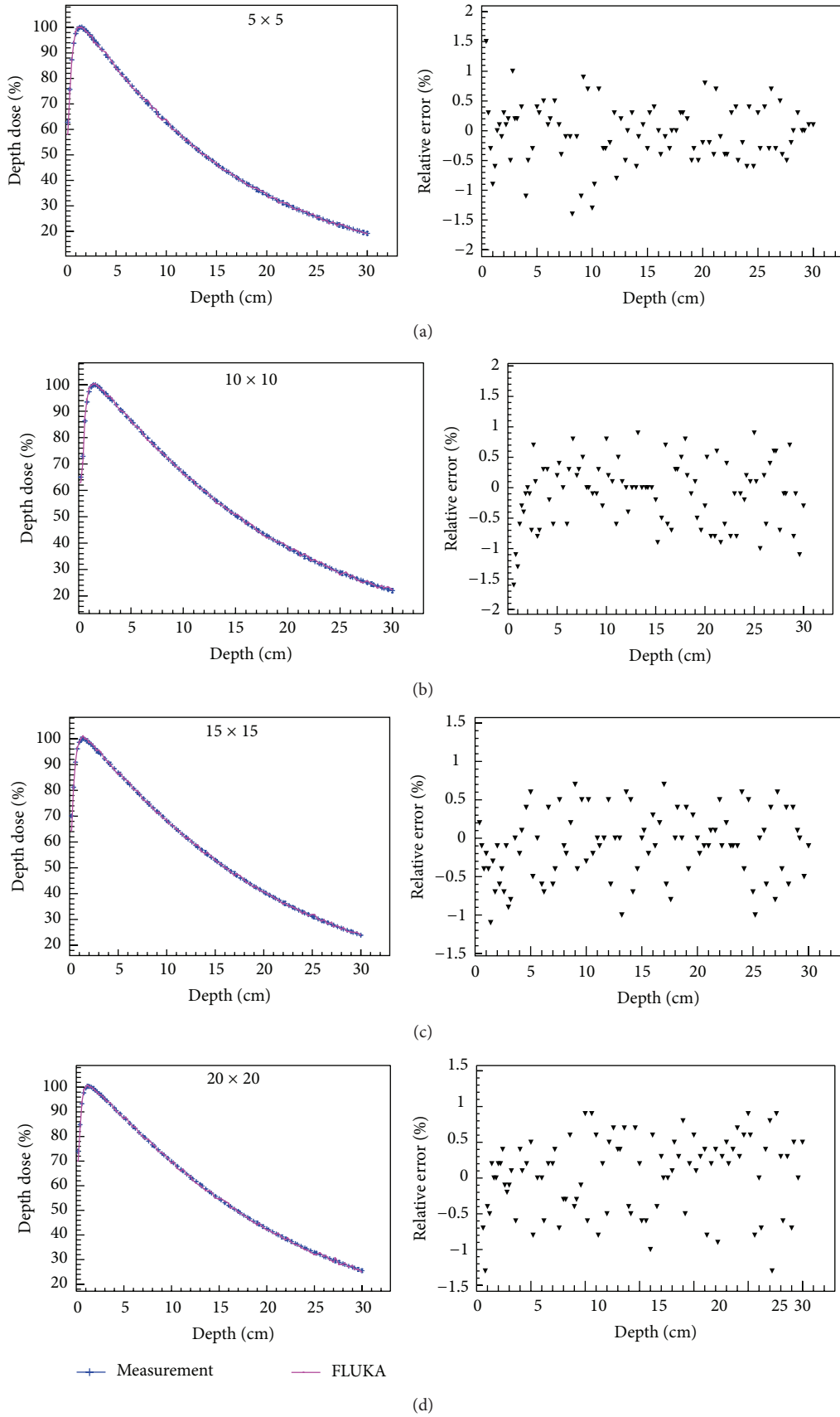
FIGURE 2: Comparison of calculated and measured percentage depth dose for 6 MV photon beam for field sizes 5 \times 5 cm 2 (a), 10 \times 10 cm 2 (b), 15 \times 15 cm 2 (c), and 20 \times 20 cm 2 (d). Relative error is shown on right side.
