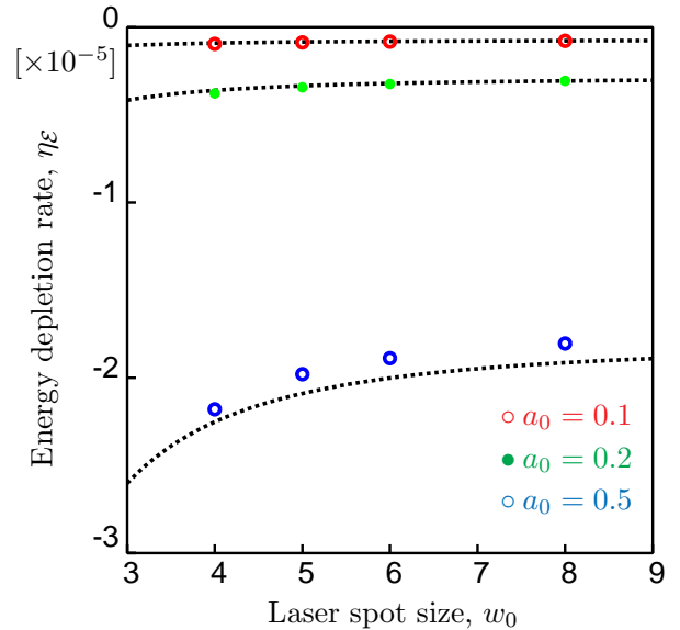
FIG. 1. Initial energy depletion rate, \eta_{\mathcal{E}} , as a function of the laser spot, w_0 , for different values of the normalized laser strength, a_0 = 0.1 (red circles), a_0 = 0.2 (green dots), and a_0 = 0.5 (blue circles). The longitudinal laser profile is Gaussian with L = 2 , and k_0/k_p = 20 . The black dotted lines are the theoretical predictions Eq. (17).
