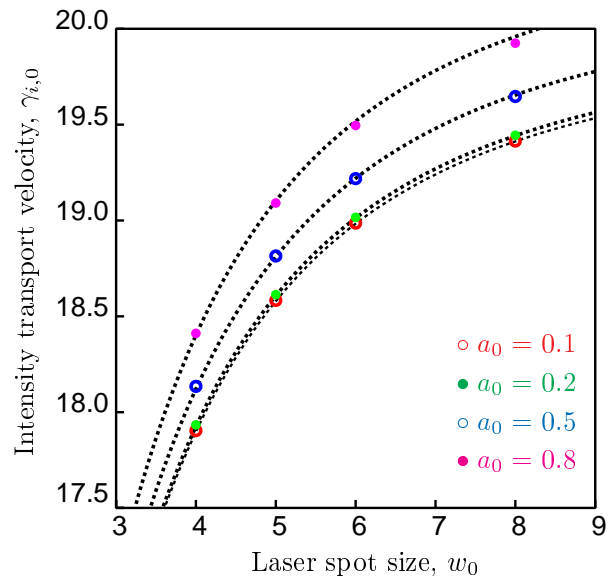
FIG. 3. Lorentz factor of the initial intensity transport velocity, \gamma_{i,0} , as a function of the laser spot, w_0 , for different values of the normalized laser strength, a_0 = 0.1 (red circles), a_0 = 0.2 (green dots), a_0 = 0.5 (blue circles), and a_0 = 0.8 (purple dots). The longitudinal laser profile is Gaussian with L = 2 , and k_0/k_p = 20 . The black dotted lines are the theoretical predictions Eq. (29).
