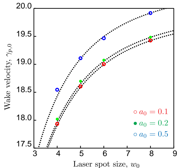
FIG. 4. Lorentz factor of the initial wake velocity, \gamma_{p,0} , as a function of the laser spot, w_0 , for different values of the normalized laser strength, namely a_0 = 0.1 (red circles), a_0 = 0.2 (green dots), and a_0 = 0.5 (blue circles). The longitudinal laser profile is Gaussian with L = 2 , and k_0/k_p = 20 . The black dotted lines are the theoretical predictions Eq. (42).
