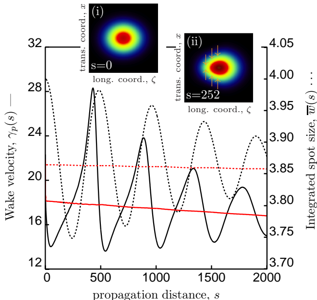
FIG. 5. Evolution of the wake phase velocity, \gamma_p(s) (black solid line) and normalized-intensity-weighted laser radius \bar{w}(s) (black dashed line), for a Gaussian laser driver with a_0 = 0.5 , w_0 = 4 , and f(\zeta) = \exp(-\zeta^2/L^2) with L = 2 . The laser is linearly matched in a parabolic plasma channel, and k_0/k_p = 20 . The two insets show snapshots of the laser envelope for two propagation distances: (i) s = 0 and (ii) s = 252 , illustrating the compression of the laser driver in the region towards the back of the pulse. The red solid line and the red dashed line show, respectively, the evolution of the wake phase velocity and laser radius for a “super-matched” driver.
