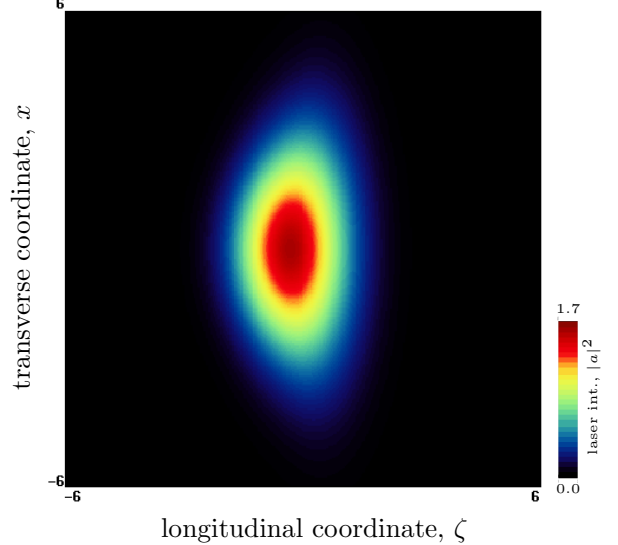
FIG. 6. Normalized laser intensity field |\hat{a}(x, y = 0, \zeta)| for a “super-matched” laser pulse driver in a parabolic plasma channel. The form of the laser envelope is given in Eq. (A2), with a_0 = 1 , and where we choose f(\zeta) = \exp(-\zeta^2/L^2) , with L = 2 . The function g(\zeta, r) is the solution of Eq. (A7) with q = 0 and R = 5 .
