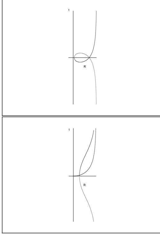
FIGURE 1. H = \frac{1}{2} : the profile curve in the immersed and embedded case ( R = \tanh \rho/2 ).
