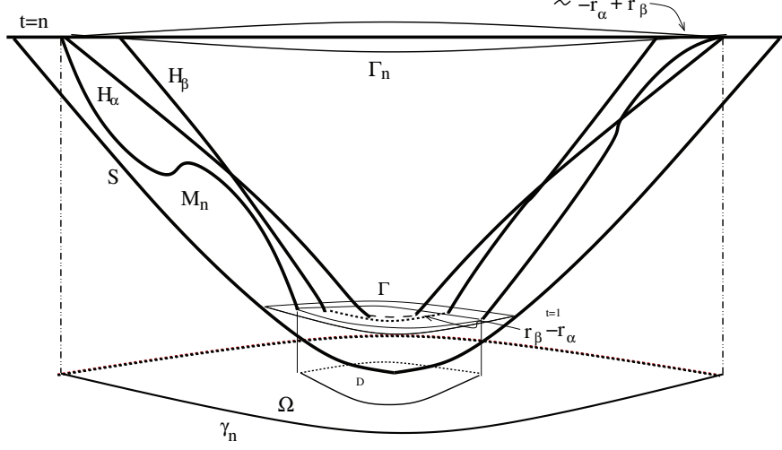
FIGURE 3. Proof of Theorem 3.4
