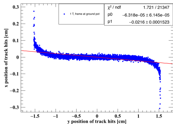
Figure 10. Projection of the track on the middle module. The anode and the mesh is at ground potential and mesh is at -380V.
