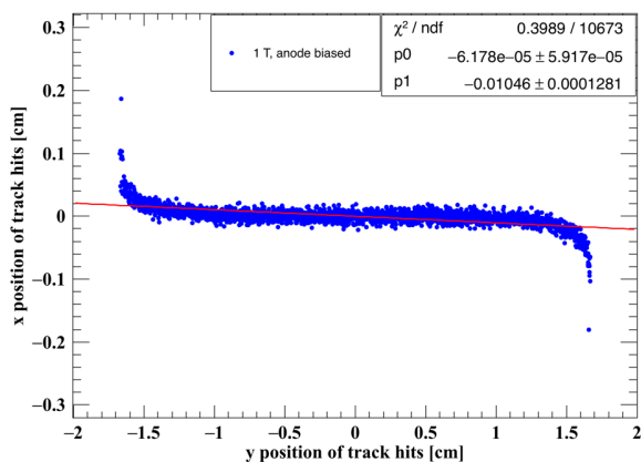
Figure 9. Projection of the track on the middle module. The anode is at +380V and mesh is at ground.
