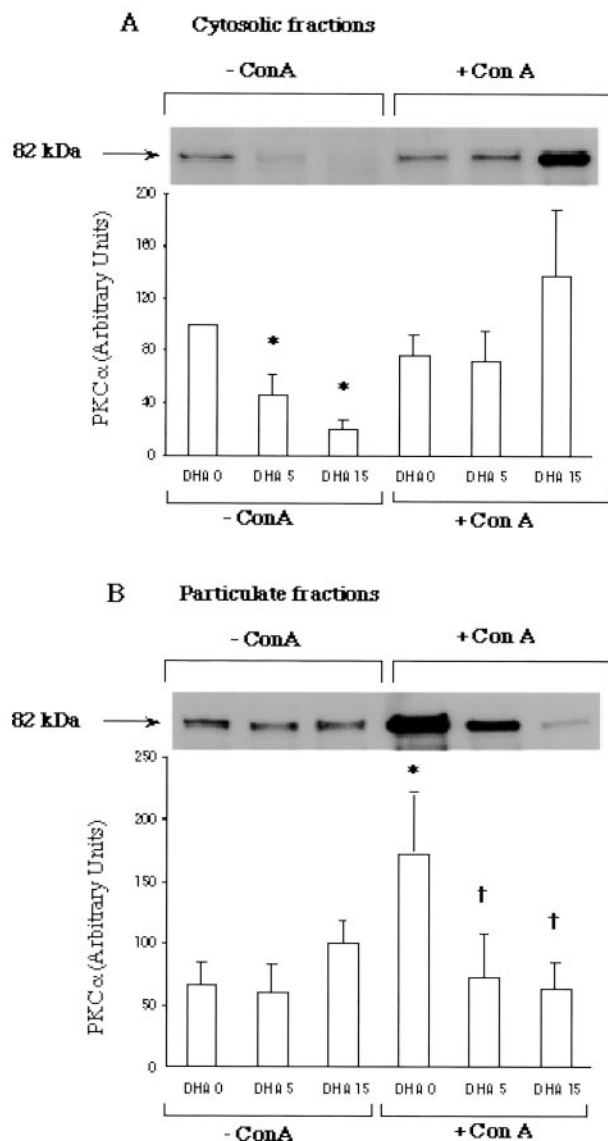
FIG. 3. Effect of DHA on the translocation of PKCα in human PBMC. PBMC were incubated for 2 h with 5 μM HSA or with 5 or 15 μM of DHA bound to HSA. Cells were then incubated for 30 min in the absence or presence of ConA (5 μg/10 6 cells). At the end of incubation, cells were lysed, and the cytosolic and particulate fractions were separated by ultracentrifugation. Cytosolic (A) and particulate (B) proteins (8 μg per lane) were analyzed by Western blotting, using an anti-PKCα monoclonal antibody for immunodetection. Spots were analyzed by videodensitometry. Bar diagrams show results expressed as arbitrary units normalized to values obtained in the cytosol of control unstimulated cells and are means ± S.D. of five separate experiments. *, significantly different from non-enriched unstimulated cells (DHA 0, -ConA) p < 0.05 ; †, significantly different from non-enriched stimulated cells (DHA 0, +ConA) p < 0.05 . Blots shown in the upper part of the two panels are from one typical experiment.
