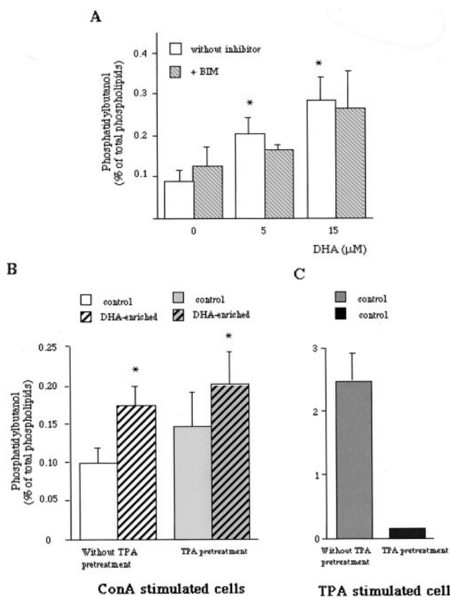
FIG. 4. The DHA-induced PLD activation in ConA-stimulated PBMC is independent of PKC. A, [ ^3\text{H} ]arachidonate-labeled PBMC were incubated for 2 h with 5 \mu\text{M} HSA or with 5 or 15 \mu\text{M} of DHA bound to HSA. Cells were then incubated in the absence or presence of 1 \mu\text{M} BIM for 30 min at 37 ^{\circ}\text{C} and further stimulated with ConA (5 \mu\text{g}/10^6 cells), in the presence of 1% butanol for 30 min. Results are expressed relative to the radioactivity incorporated in total phospholipids and are means \pm S.E. of four separate experiments. Data were analyzed by ANOVA, and means were compared by a protected t test. *, significantly different from control non-enriched cells. p < 0.05 . B, [ ^3\text{H} ]arachidonate-labeled control or DHA-enriched (5 \mu\text{M} ) PBMC were incubated in the absence or presence of 100 nM TPA for 14 h and then stimulated with ConA (5 \mu\text{g}/10^6 cells) in the presence of 1% butanol for 30 min. Results are expressed relative to the radioactivity incorporated in total phospholipids and are means \pm S.E. of five separate experiments. Data were analyzed by ANOVA, and means were compared by a protected t test. *, significantly different from control non-enriched cells without TPA pretreatment. p < 0.05 . C, [ ^3\text{H} ]arachidonate-labeled control PBMC were incubated in the absence or presence of 100 nM TPA for 14 h and then stimulated with 10 nM TPA in the presence of 1% butanol for 30 min. Results are expressed relative to the radioactivity incorporated in total phospholipids and are means \pm range of two separate experiments.
