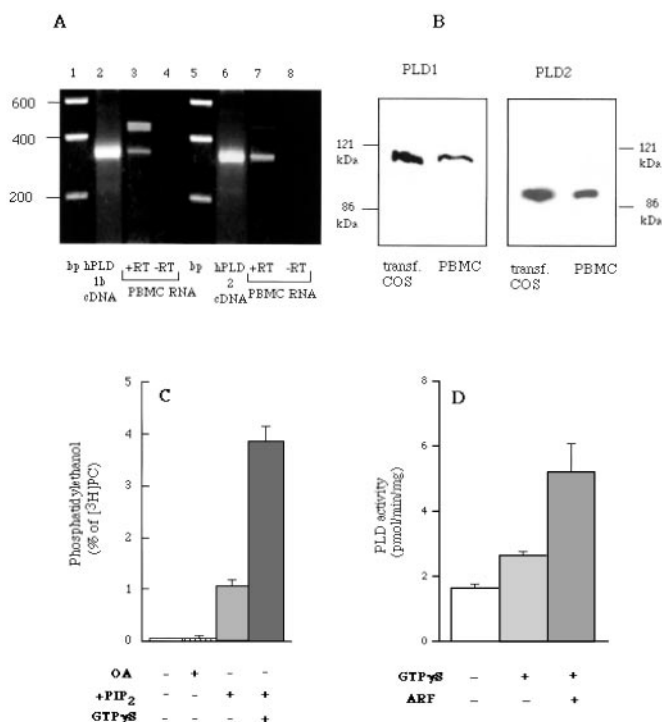
FIG. 2. Characterization of PLD in human PBMC. A, RT-PCRs were carried out as described under "Experimental Procedures" using specific primers for PLD1, which allowed us to discriminate the splice variants PLD1a and -1b (lanes 2–4) and primers for PLD2 (lanes 6–8). Positive controls were obtained by using pCDNA3 plasmids carrying hPLD1b (lane 2) and hPLD2 (lane 6) cDNAs as templates. Negative controls were obtained by using PBMC RNA untreated by reverse transcriptase (lanes 4 and 8). Lane 3, the larger product of 446 bp and the smaller one of 332 bp derived from PLD1a and PLD1b, respectively; lane 6, the band at 329 bp has the expected size for amplification of a PLD2 transcript. B, total cell lysates from 6 \times 10^6 PBMC were subjected to SDS-PAGE and analyzed by Western blotting using PLD1 and PLD2 antisera. Lysates from COS-1 cells transfected with pCDNA3-hPLD1b and pCDNA3-hPLD2 were used as positive controls. C, aliquots of cell lysates ( 8 \times 10^6 cells) were added to a reaction mixture containing 2.7 mM [ 3 H]DPPC in the absence (–) or presence (+) of 2 mM sodium oleate or to reaction mixtures containing 8 μM [ 3 H]DPPC in the absence (–) or presence (+) of 12 μM PIP 2 , with or without 50 μM GTPγS. [ 3 H]Phosphatidylethanol was separated by TLC. D, aliquots of the 100,000 × g pellet fraction (from 8 \times 10^6 cells) were added to reaction mixtures containing substrate phospholipid vesicles (PE/PIP 2 /PC, 16:1.5:1) and incubated at 37 °C for 30 min in the absence (–) or presence (+) of 50 μM GTPγS with or without recombinant ARF. [ 3 H]Choline released from dipalmitoylphosphatidyl[methyl- 3 H]choline was measured as described under "Experimental Procedures." Data are means ± S.E. of three separate experiments.
