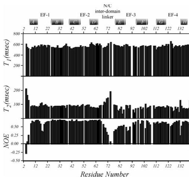
FIG. 2. Plot of backbone amide ^{15}\text{N} T_1 , T_2 , and heteronuclear ^{15}\text{N}(^1\text{H}) -NOE values versus residue number for wild-type Cdc4p. The N and C termini and the linker region connecting the two domains of the protein exhibit conformational flexibility on a sub-nanosecond time scale as indicated by anomalously high T_2 and low heteronuclear NOE values. Residues within the loop regions, particularly between helices A and B and helices E and F, also show evidence of conformational mobility. The positions of the eight helices are indicated above the figure with cylinders.
