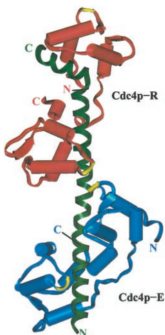
FIG. 4. A proposed model of interallelic complementation in which two Cdc4p proteins bind to the S1 neck region of the myosin heavy chain. The figure illustrates Cdc4p, modeled according to the crystallographically determined structure of the scallop muscle ternary complex (42) as the equivalent of an RLC (red) and ELC (blue), bound to the neck region of the myosin heavy chain (green). Note the different conformations of the ELC and RLC with respect to interhelical angles and that both light chain-heavy chain and light chain-light chain interactions are required to stabilize the complex. The positions of Gly-19 and Gly-107 in Cdc4p are highlighted in yellow. According to this model of interallelic complementation, single point mutations, such as G19E or G107S, disrupt the complex in part by destabilizing necessary interactions between Cdc4p in the two light chain positions, leading to a conditionally lethal phenotype. However, in a diploid cell expressing copies of both mutant alleles, a wild-type interface exists between Cdc4p-G19E in the RLC position and Cdc4p-G107S in the ELC position, thereby allowing formation of a ternary complex as required for cytokinesis.
