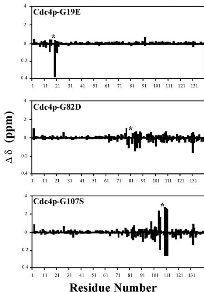
FIG. 3. Amide chemical shift perturbations indicate that only small structural perturbations result from three amino acid substitutions that lead to a temperature-dependent phenotype for Cdc4p. Shown are plots of the absolute values of the chemical shift differences between the ^{15}\text{N} (upwards bars) and ^1\text{H} (downwards bars) chemical shifts of corresponding amides in each mutant protein versus wild-type Cdc4p. The position of each amino acid substitution is indicated with an asterisk. Small chemical shift differences ( <0.03 ppm in ^1\text{H} and <0.25 ppm in ^{15}\text{N} ), as well as changes near His-131, are attributed to slight variations in sample buffer conditions.
