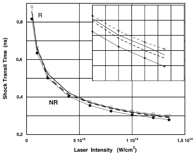
Fig. 6. Shock transit time in a 8.5 \mu\text{m} Al step for radiative (R) and non-radiative (NR) cases as a function of laser intensity. The curve C corresponds to the shock transit time obtained in the non-radiative case when a reduction of the pressure according to the radiative case is adopted (see Fig. 5). Curve D is obtained scaling the non-radiative values by the square root of the non-radiative and radiative pressures ratio. The inset on top-right shows the detail at high laser intensities.
