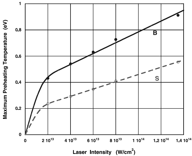
Fig. 3. The maximum value of the preheating temperature at the rear surfaces of base and step, 8 and 8.5 \mu\text{m} , as a function of laser intensity. The values are taken just before the respective shock breakouts.
