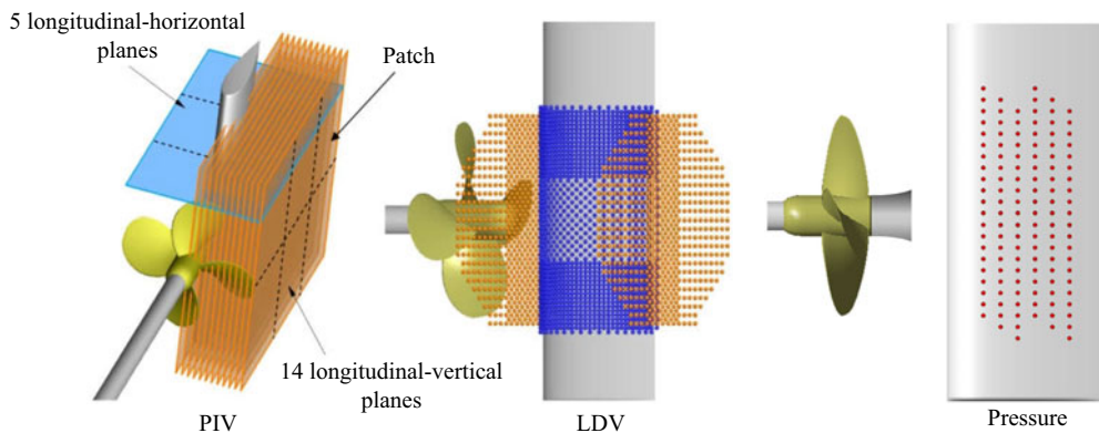
FIGURE 6. Measurement grids.
