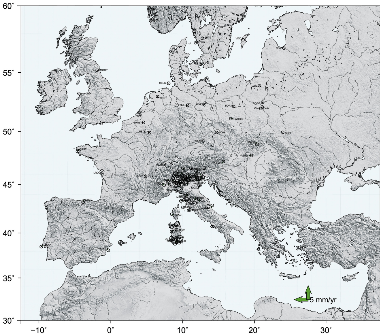
Fig. 2 – Residual horizontal intra-plate Eurasian velocities of the 111 sites of our solutions with residual velocity values <0.95 mm/yr; for the sake of convenience, the authors omit the corresponding data table. Uncertainty ellipses represent the 68% level of confidence.
