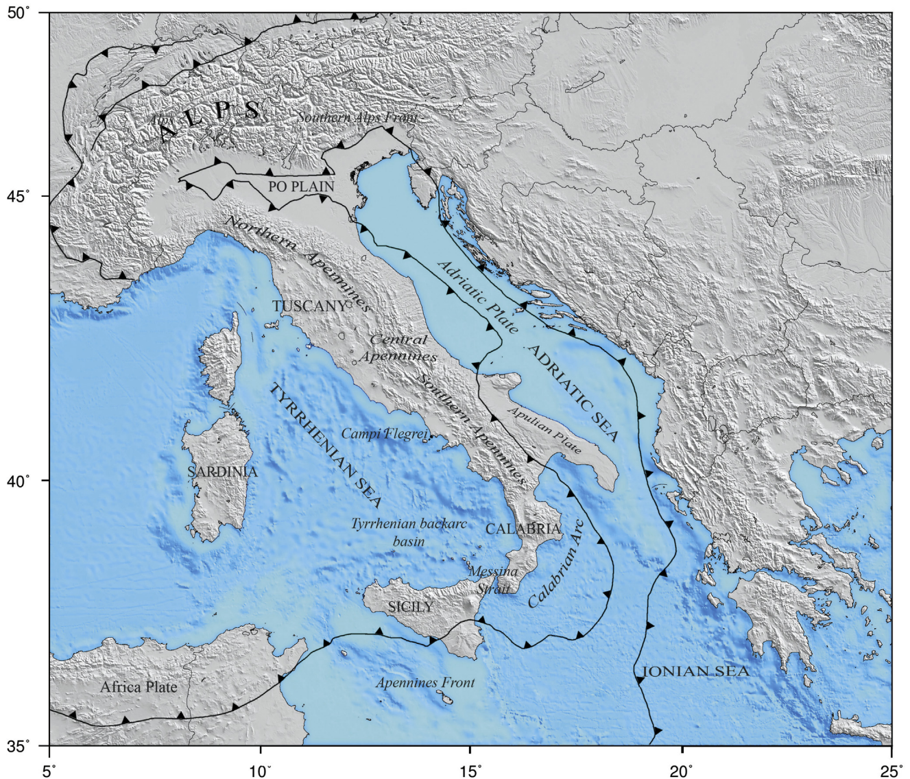
Fig. 3 – The geodynamic map of the Italian Peninsula; major tectonic structures are represented (modified from reference [45]).
