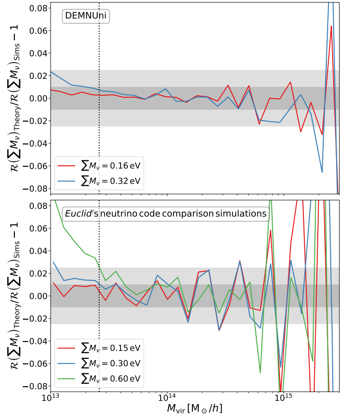
Fig. 17. Accuracy of the model presented in Castorina et al. (2014) in accounting for the impact of massive neutrinos on the HMF. We compare the ratio of the HMF with massive neutrinos to the corresponding massless neutrinos counterpart, assuming the model of Castorina et al. (2014) divided by the same quantity as observed in two independent external simulations: DEMNUni (top) and the Open-GADGET subset of Euclid 's neutrino code comparison simulations (bottom). See the definition of \mathcal{R} in Eq. (20).
