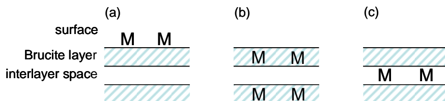
Figure 11 Immobilization of metal species (M) on the surface (a), in the Brucite layer (b) and within the interlayer space (c) of the hydrotalcite.
