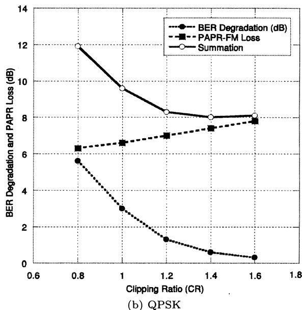
Fig. 6. BER degradation and PAPR-FM loss as a function of CR.
