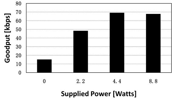
Fig. 15 Evaluation result of goodput for supplied power.
