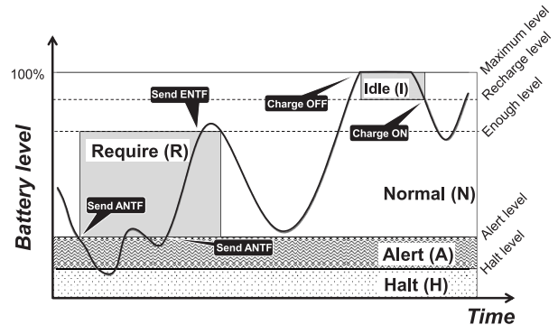
Fig. 3 Diagram of battery level variation with time.
