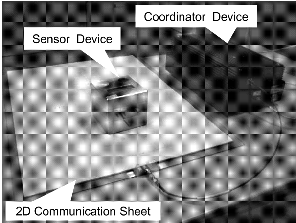
Fig. 16 Experiment setup.
