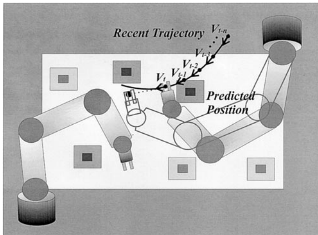
Figure 10. Predicted image superimposed on the delayed robot.
