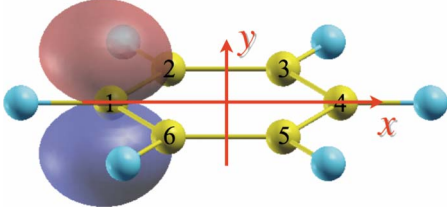
FIG. 2. (Color online) The MLWF around the carbon atom one obtained for a Bz molecule is plotted with \text{isovalue}=0.1 . All six MLWFs are identical and their centers are shifted from nearby C atomic sites along each C-H bond by about 0.07 \text{ \AA} .
