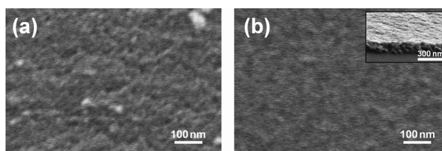
FIG. 10. SEM images of the AZO thin film (a) before and (b) after the annealing. The inset in (b) shows the cross-sectional SEM micrograph of the annealed film.
