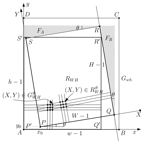
Fig. 2 Two rectangles G_{wh} and R_{WH} .
