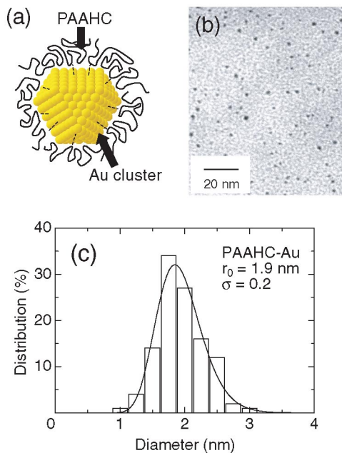
FIG. 1 (color online). (a) Schematic of PAAHC-Au nanoparticles. (b) TEM image of Au nanoparticles protected by PAAHC. Mean diameter of the sample is 1.9 nm. Scale bar is shown in the image. (c) Size distribution of PAAHC-Au nanoparticles. The solid line represents the fitting curve assuming the log-normal function f(r) = \frac{1}{\sqrt{2\pi}r\sigma} \exp\left(-\frac{(\ln r - r_0)^2}{2\sigma^2}\right) where r is the particle diameter. The fitting results of parameters are the mean particle diameter r_0 = 1.9 nm and the standard deviation \sigma = 0.2 nm.
