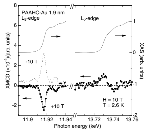
FIG. 2. XMCD and XAS spectra at the Au L_{3-} and L_{2-} edge with an applied magnetic field of 10 T. The XMCD and XAS spectra include a same scale factor so that the height of the edge jumps of the XAS spectra (solid lines) are unity. Solid lines with closed circle symbols represent an XMCD spectrum with an applied magnetic field of 10 T, while the dotted line indicates an XMCD spectrum in a magnetic field applied in the opposite direction, implying the observed signal is not an artificial effect.
