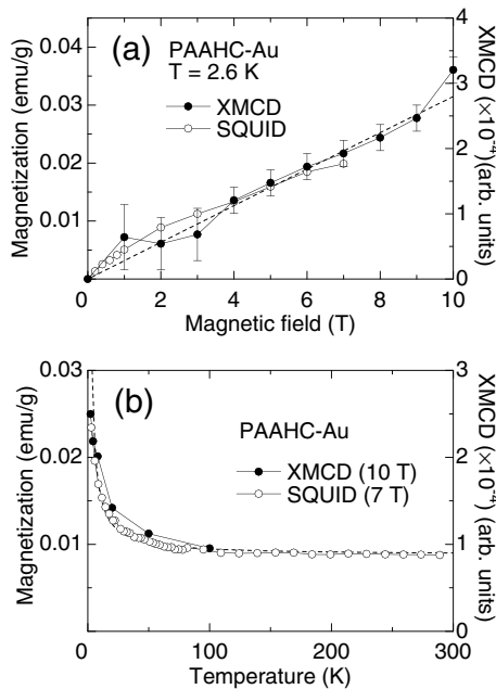
FIG. 3. (a) ESM of PAAHC-Au as a function of the applied magnetic field and magnetization process obtained by SQUID magnetometer. The integral of the peak intensity yields similar results. Dotted line is the fit to the data assuming a Langevin function plus a linear field-dependent term. (b) Temperature dependence of the XMCD peak intensity at 10 T recorded at the Au L_3 -edge and temperature variation of the magnetization measured by SQUID magnetometer at 7 T. Dotted line is the fit to the data assuming \chi(T) = N\mu L(x)/H + \chi_{\text{Pauli}} . Solid lines are guides for the eye.
