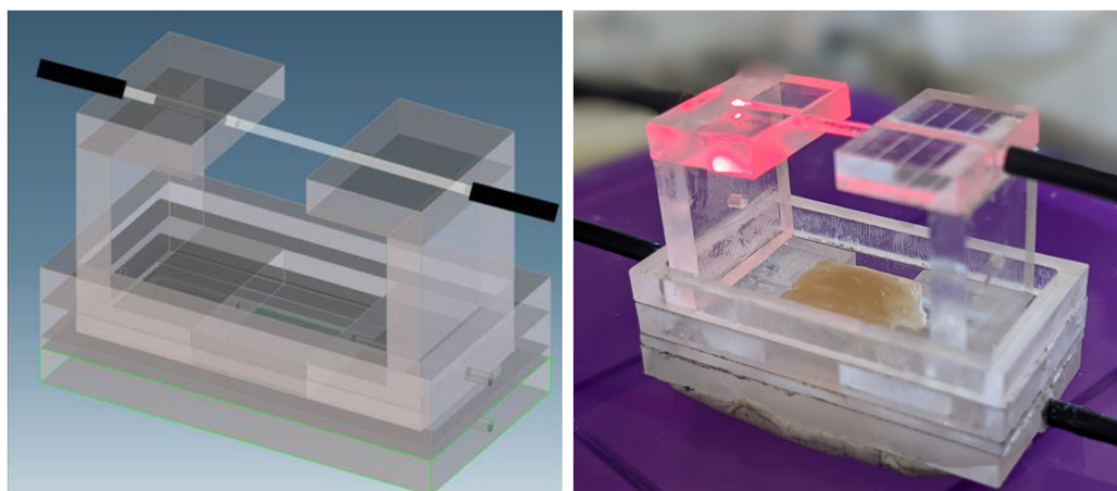
Figure 4. Fiber-optic sensor based on mobile platforms. In the (left panel), the 3D model shows the discontinuity between both stripped parts of the optical fiber when they are separated. The fabricated sensor includes the guides along which both PMMA platforms move. In the (right panel), the cardiac tissue placed on the sensor to measure the stretch is shown. The tissue sample is located in contact with the medium, which does not influence the stretch measurement since this is based on the upper fibers.
