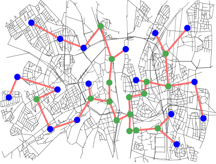
Figure 2: Location of BSs and topology of the backhaul.
