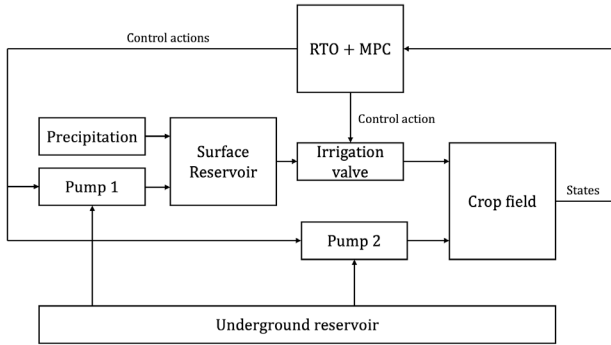
Fig. 1. A schematic of interaction between surface-groundwater reservoirs and crop field with the controller.
