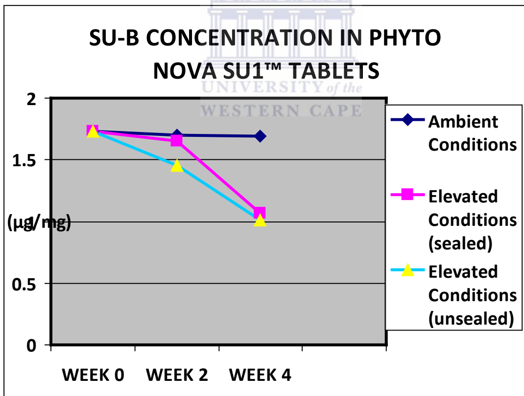
Figure 15: SU-B concentration in Phyto Nova Sutherlandia SU1™ tablets and Promune™ capsules during 4 weeks storage under ambient and elevated temperature and humidity conditions
