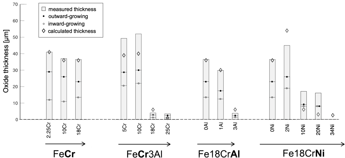
Figure 5.4: Summary of the measured oxide scale thicknesses for all model alloys exposed for 48 hours in 5% O_2 + 95\% N_2 + 1 \text{ mg/cm}^2 K_2CO_3(s) at 600 °C, including estimated thicknesses, calculated from mass gain data, ( \diamond ). Note that the oxide scale formed on the Fe18Cr34Ni alloy was not examined in cross section.
