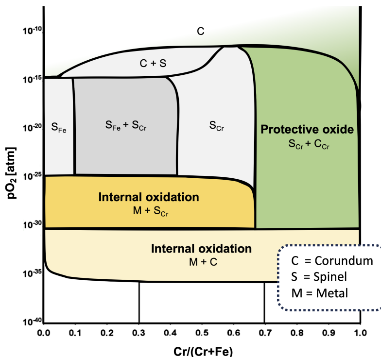
Figure 2.4: Phase diagram for the FeCrO system at 600\text{ }^\circ\text{C} that can be used to predict the phases that would form at equilibrium for certain pO_2 -levels and concentrations of Cr. C_i =corundum-type oxide ( i=Fe, Cr ), S_i =spinel type oxide ( i=Fe, Cr ), M =metal (BCC or FCC).
