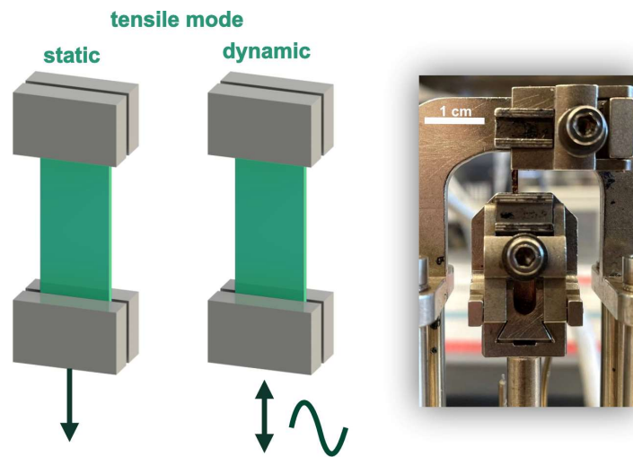
Figure 3.2. Schematic of the working principles of DMA in static or dynamic mode. A picture of a free-standing sample mounted in the DMA clamps.
