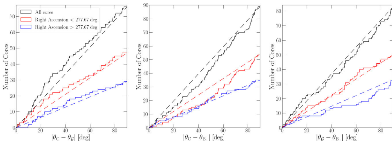
Figure 10. Relative alignment of \theta_C , \theta_G , and \theta_{B_\perp} following the same formatting as Fig. 9. In this case, the red or blue solid curve and dashed line represent cores below or above \alpha = 277.67^\circ in Serpens, respectively.
