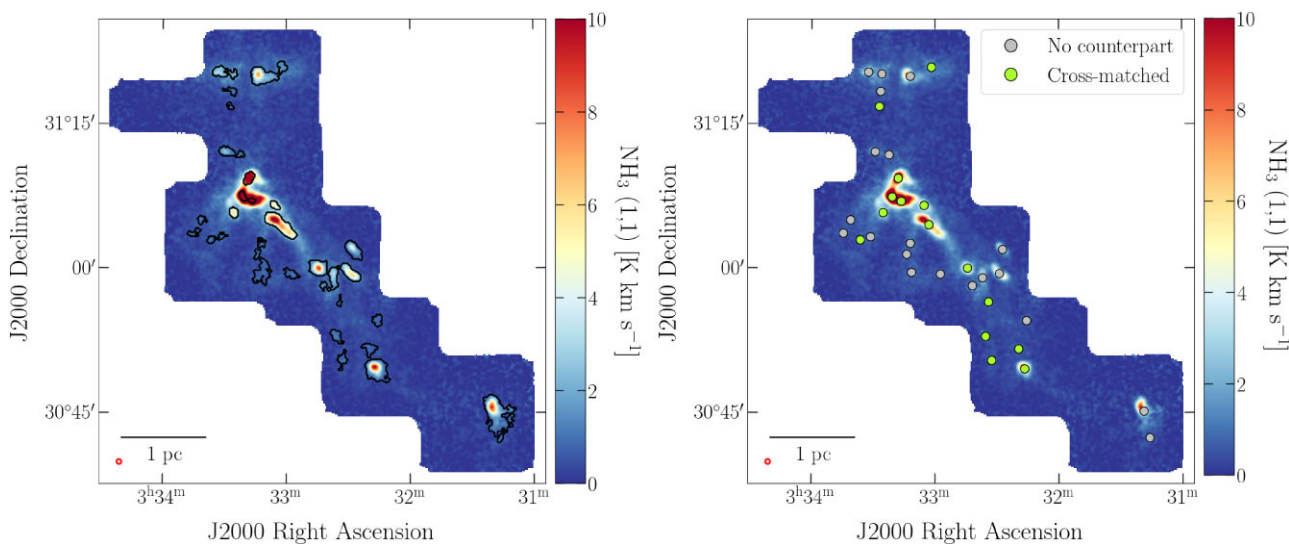
Figure 1. (Left) \text{NH}_3 (1,1) integrated intensity map of the B1 Perseus region with identified dense cores (classified as leaves in astrodendro ) outlined in black. There are 35 identified cores in this region of the GAS data. A scale bar depicting the angular size of 1 pc at the distance of the B1 Perseus region is presented in the bottom left corner. Also in the bottom left corner is a red ellipse representing the 32'' beam size of the GAS data. (Right) The same \text{NH}_3 (1,1) integrated intensity map as on the left is presented after applying the cross-matching algorithm. \text{NH}_3 cores that were successfully cross-matched are overlaid as green circles and cores with no identified continuum counterpart are plotted as grey circles. In this region, 15 out of 35 dense cores identified in GAS were uniquely cross-matched with a continuum counterpart in HGBS data.
