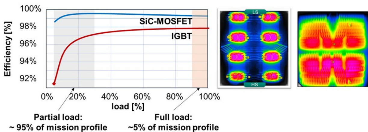
Figure 2-4 | Energy efficiency of SiC-MOSFET vs Silicon IGBT based main drive inverters as a function of the electrical current through the inverter (“load”)
