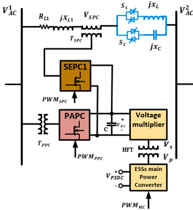
Fig. 2. Proposed UIPC topology.
