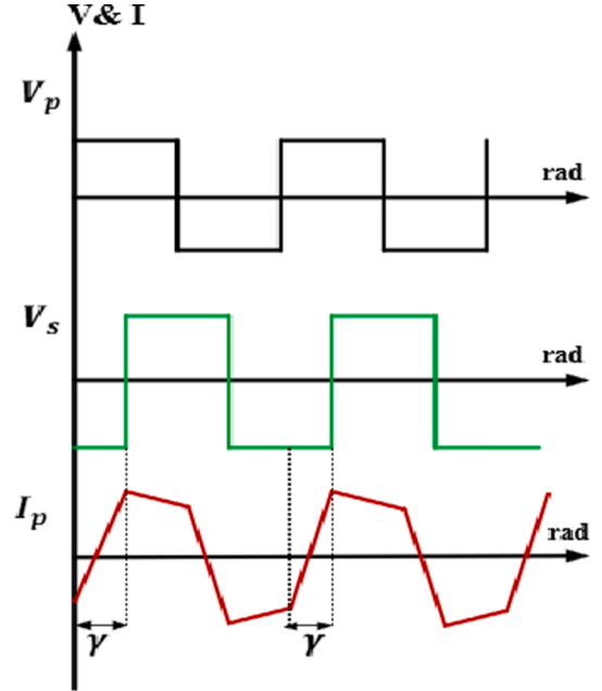
Fig. 3. The voltages and current of HFT.
