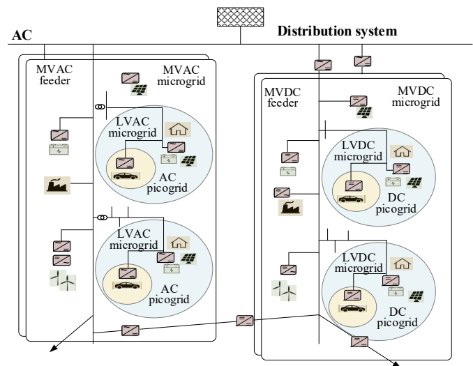
Fig. 1. Structure of the modern power electronics-based power system [5].
