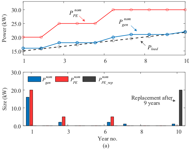
Fig. 6. Case study results: Optimum size of PV arrays P_{gen}^{nom} and PV inverters P_{PE}^{nom} over the planning horizon T_{PH} of 10 years for the input load demand P_{load} : (a) with included power electronics reliability into decision-making process, and (b) without included power electronics reliability.
