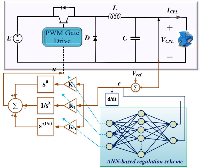
Fig. 3. Diagram of ANN-based Hybrid controller applied to a DC-DC converter
