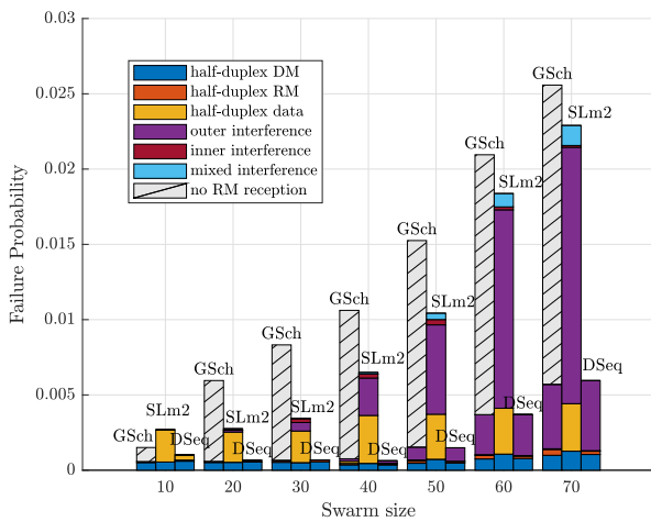
FIGURE 6. Failure probability and the causes of data transmission failures (half-duplex of DM, RM and data, inner, outer and mixed interference, and no RM reception) for three resource allocation schemes (SLm2, DSeq and GSch).
