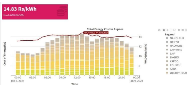
Fig. 9. Generation cost for each power source and associated WACG of each hour
