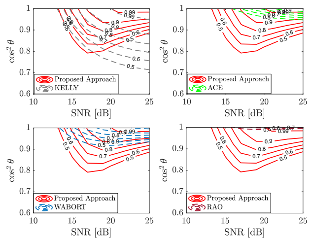
Fig. 15. Mesa plots of the double-well detector compared to Kelly, ACE, WABORT and RAO detectors for N = 4 , K = 8 , evaluated on the Phase One dataset.
