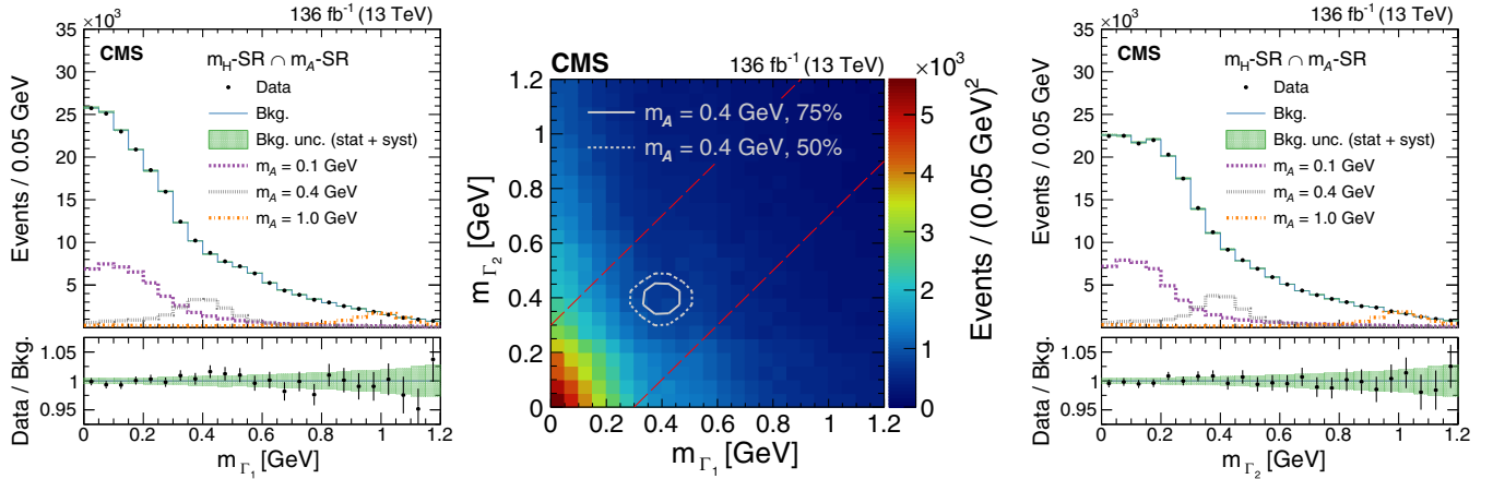
FIG. 1. Mass distributions from selected events in data. Center: the 2D- m_\Gamma distribution for data events in the m_H -SR. The red dashed lines indicate the m_{\mathcal{A}} -SR boundaries. The contours of simulated H \rightarrow \mathcal{A}\mathcal{A} \rightarrow 4\gamma events for m_{\mathcal{A}} = 0.4 GeV are plotted for 75% (solid contour) and 50% (dotted contour) of the distribution maximum. The corresponding m_{\Gamma_1} (left) and m_{\Gamma_2} (right) projections for the overlap of the m_H -SR and m_{\mathcal{A}} -SR are also shown. The data distributions (black points) are plotted against the total predicted background distributions (blue curves). The statistical uncertainties in the former are negligible and the total uncertainties in the latter are barely visible as green bands. The spectra of simulated H \rightarrow \mathcal{A}\mathcal{A} \rightarrow 4\gamma events for m_{\mathcal{A}} = 0.1 (purple dashed curve), 0.4 (gray dotted curve), and 1.0 GeV (orange dash-dotted curve) are also provided. They are each normalized to the value of \mathcal{B}(H \rightarrow \mathcal{A}\mathcal{A} \rightarrow 4\gamma) that is expected to be excluded by the background model (described under the CL_s criterion in our results) times 10^3 . The black points in the lower panels of the left and right plots give the ratios of the data to the predicted background distributions. The vertical bars represent the statistical uncertainties in the former, and the green bands represent the total uncertainty in the latter.
